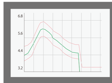
Individual torque tolerances and graph
